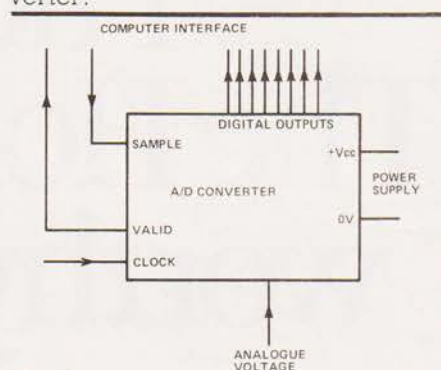
Fig. 2. Typical pin functions of an A/D converter
