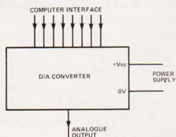
Fig. 3. Typical pin functions of a D/A converter
