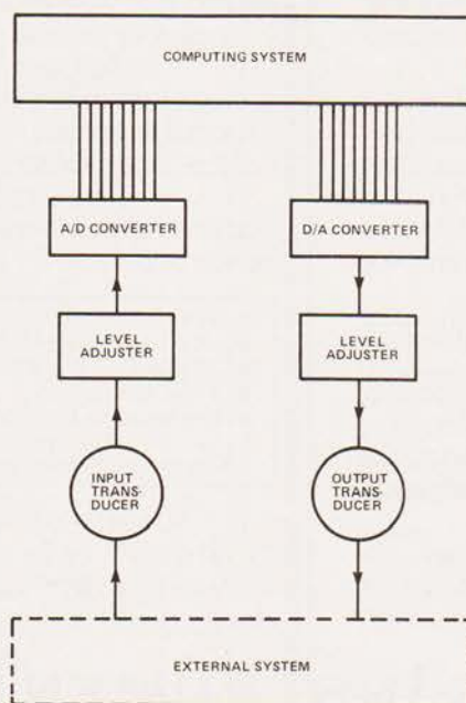
Fig. 1. Matching components
