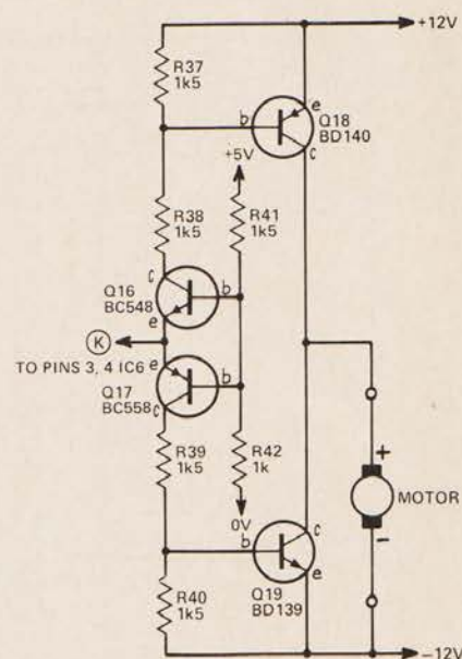
Fig. 1d. The motor drive interface.
