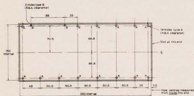
THIRD ANGLE PROJECTION all dimensions in mm
