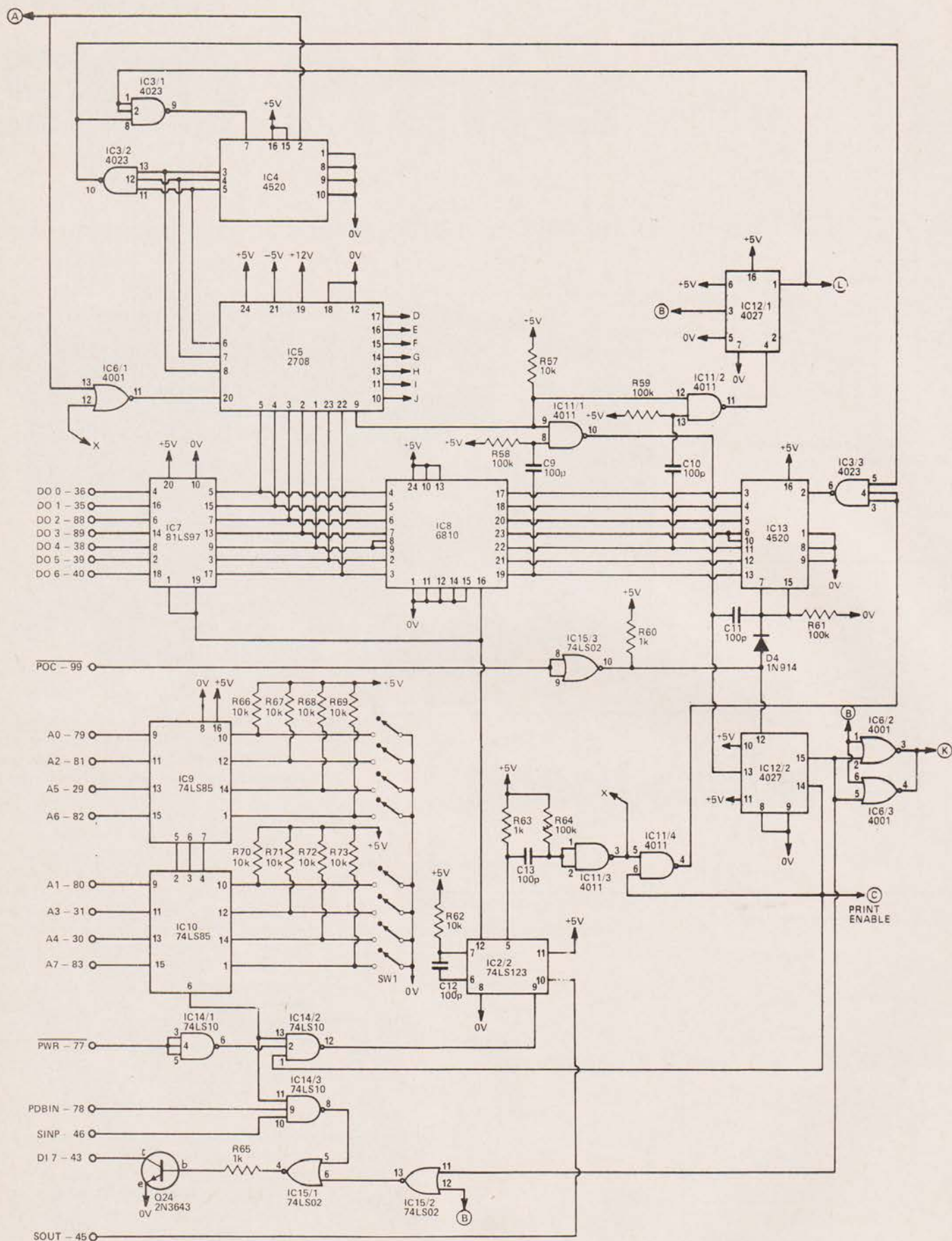
Fig. 1f. The main logic diagram.
