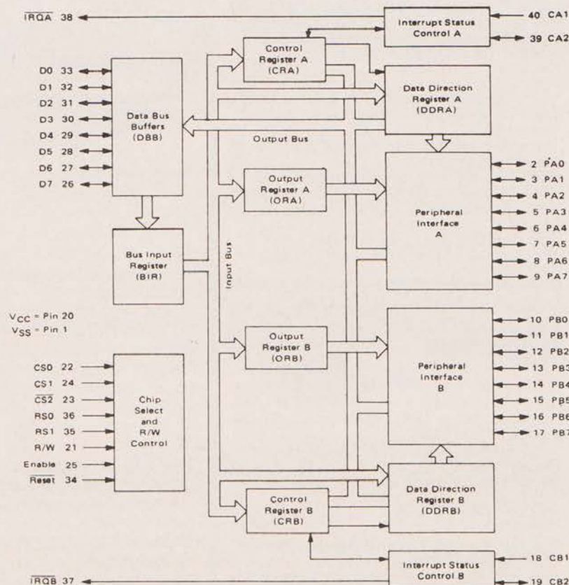
Fig 6. The Peripheral Interface Adapter provides two 8-bit bidirectional points.
